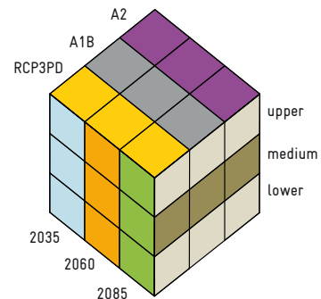
Figure 1: "Scenario cube" mapping the CH2011 scenario space. Scenarios of anthropogenic greenhouse gas emissions include A2 (high emissions, no intervention to reduce climate change), A1B (intermediate emissions, no intervention), and RCP3PD (low emissions due to an effective mitigation policy; referred to as RCP2.6 in the Fifth Assessment Report of the Intergovernmental Panel on Climate Change, here RCP3PD is used for consistency with CH2011). Time periods are 30-year averages centered on the years 2035, 2060, and 2085. Climate projections of temperature and precipitation with respect to the reference period 1980-2009 include a medium estimate, and an uncertainty range from upper to lower estimates, with an estimated 2/3 chance of covering the true temperature change, and an estimated 1/2 chance of covering the true precipitation change.
